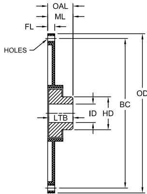
1-Piece Flange
